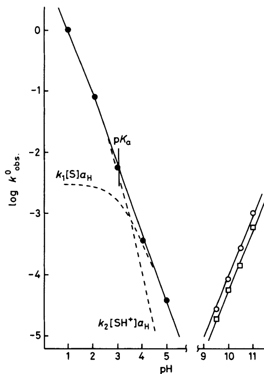
Figure 1. Rate-pH profiles for the hydrolysis of the glycosidic bond of ( 1 ) at 25 °C and ionic strength 1.0 (●) and for the disappearance (○) and glycosidic bond cleavage (□) of ( 1 ) at 40 °C and ionic strength 1.0.
